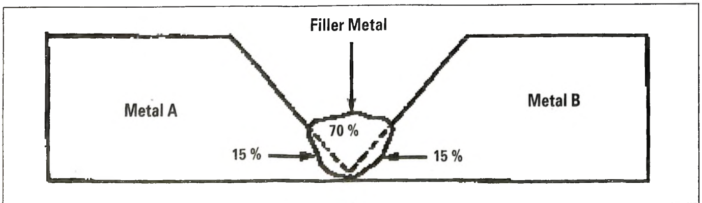
Fig. 1. Weld bead with 30% dilution, 15% from Metal A and 15% from Metal B.
