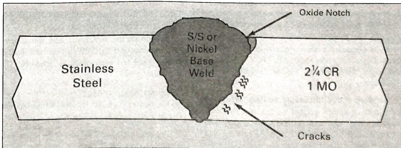
Fig. 3. Typical dissimilar-metal weld defects in boiler tubes after a long time in service.
