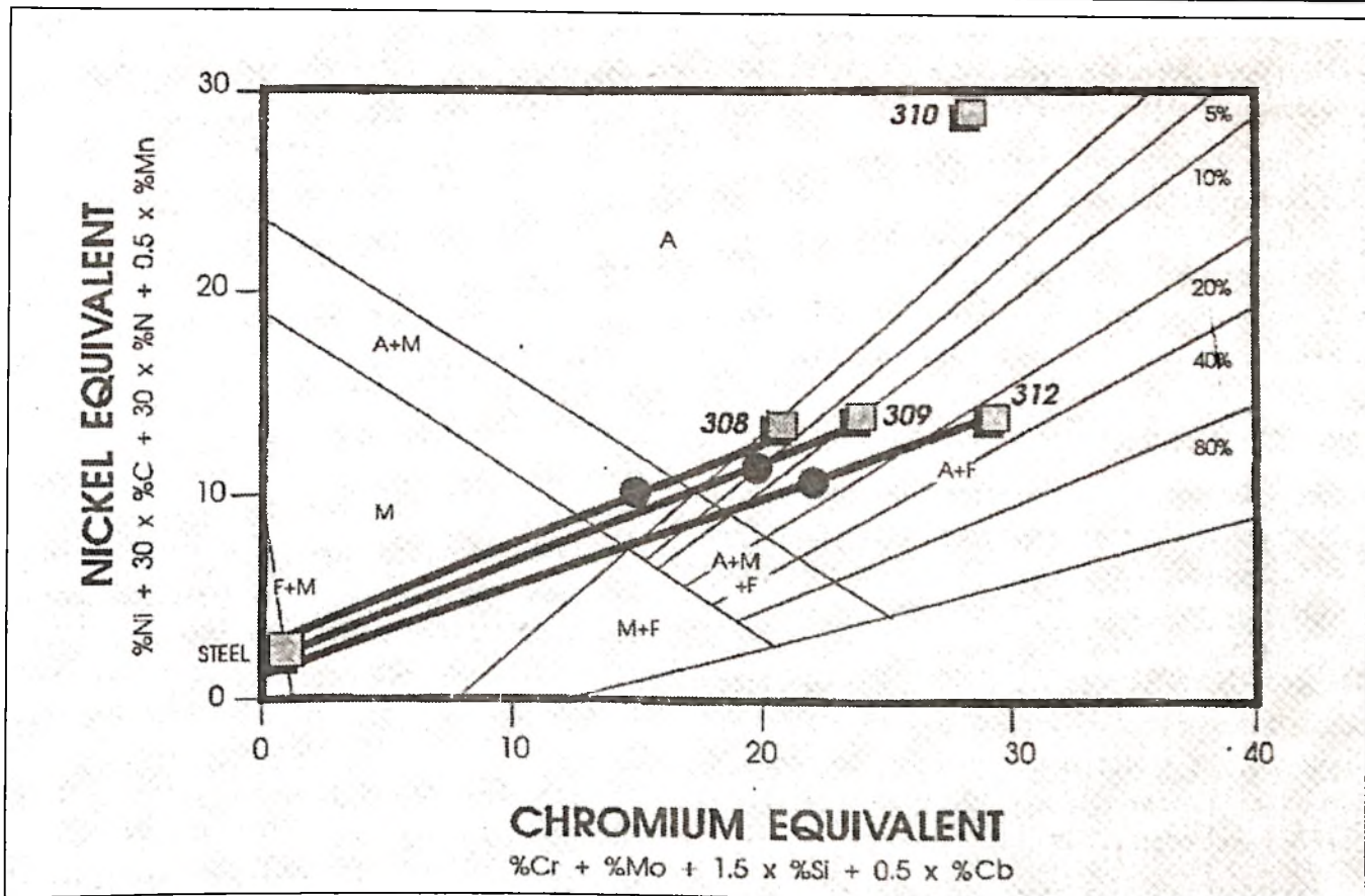
Fig. 2. Effect of 25% mild steel dilution types 308, 309, and 312 weld metals. Structure of the diluted 308 is austenite and martensite while 309 and 312 is austenite and ferrite.
