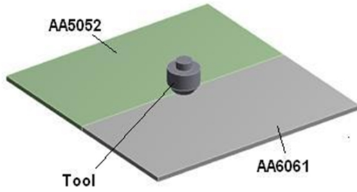
Fig 5: 3D modeling of the tool and work piece.
