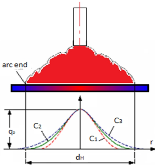
Fig 7 : 2-D Pavelic's model
