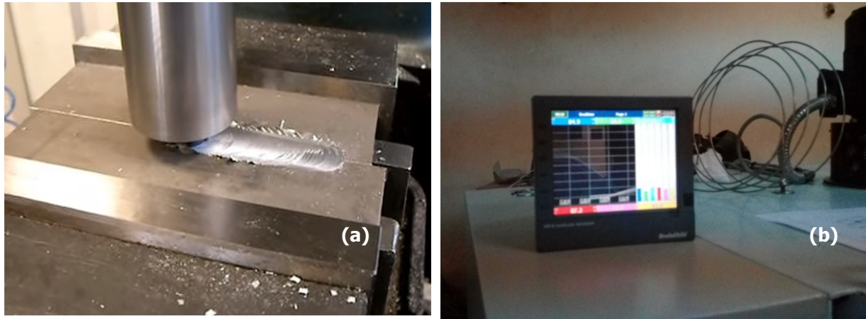
Fig 2 : a) Friction Stir Welding of AA5052-AA6061 plates with a conventional milling machine. b) Temperature – time measurement with data acquisition.
