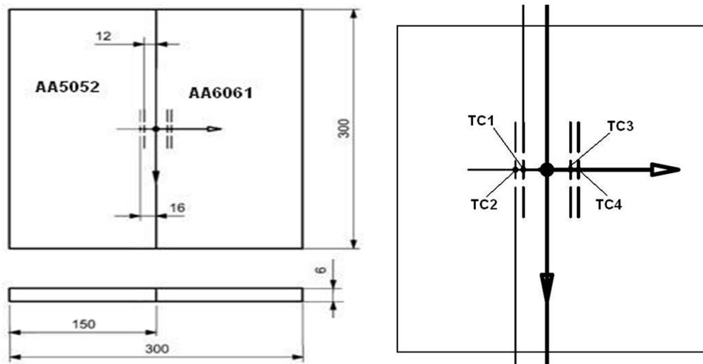
Fig 3 : Model dimension and thermocouple location.
