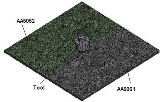
Fig 6 : Finite Element meshing of the tool and work piece
