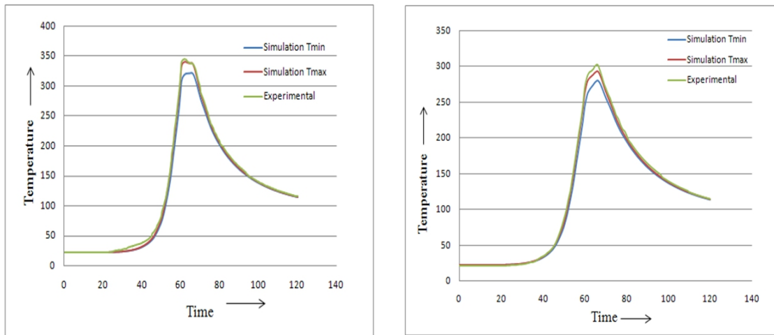
Fig 10 : Comparison between Experimental and Numerically simulated Temperature – Time curves for AA6061 plate at a distance of 12mm (left) and 16mm (right) from weld centre line.
