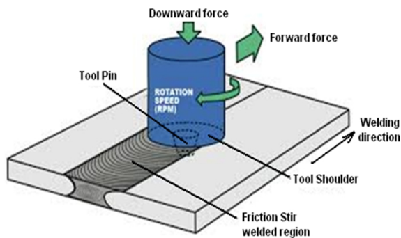
Fig 1 : Friction Stir Welding Process
