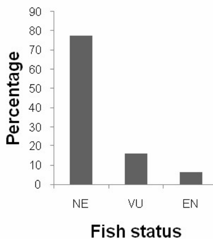
Fig. 5. Conservation categorization of fish species (as per Lakra et al. , 2010b).
