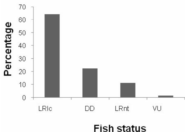
Fig. 4. Conservation categorization of fish the (as per IUCN Red list, 2011)
