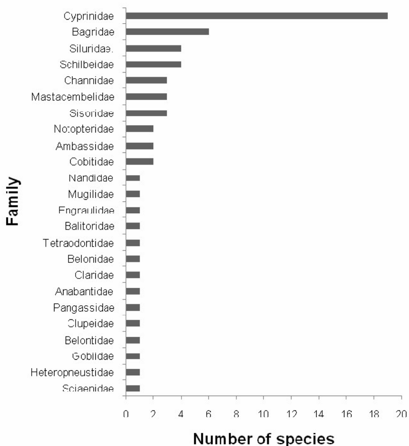
Fig. 2. Diagrammatic representation of the number of fish species occurring in each family.
