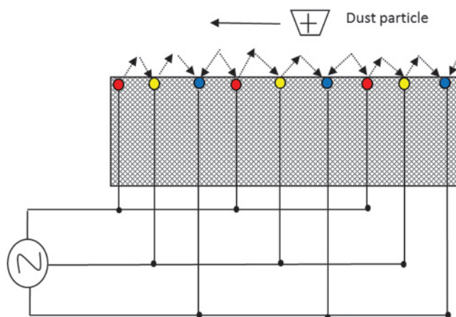
Fig.1: Three phase electric curtain
