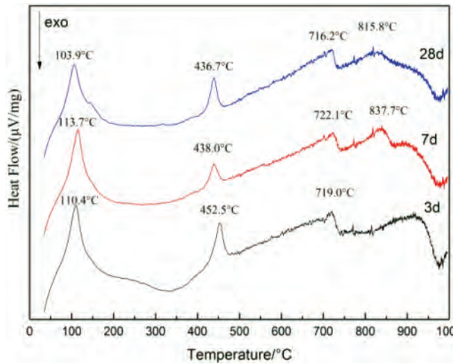
Fig.8 DSC curves of the neat paste specimen of epidote at different ages
