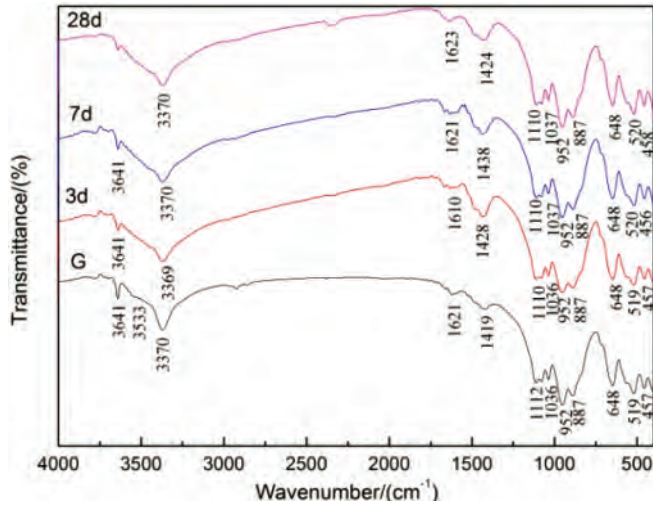
Fig.7 FT-IR spectrums of the dry mixed powder and neat paste specimen of epidote at different ages
