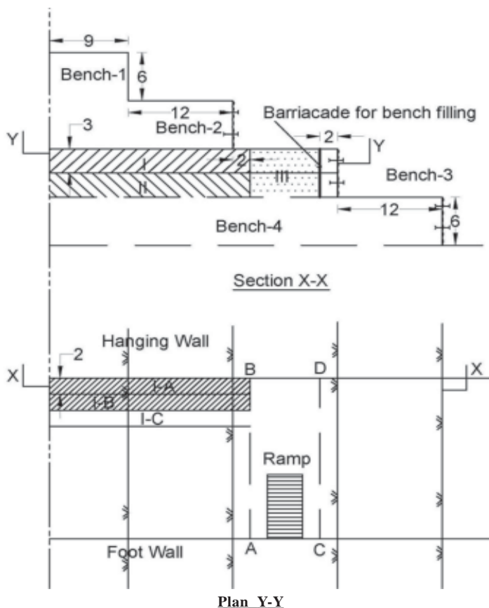
Fig.4 Plan and section of the benches showing method of UCF with CRF
