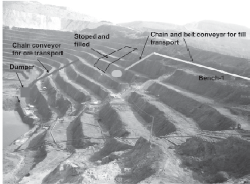
Fig.5 Schematic layout of transport of fill materials to an open pit bench and of extracted ore from at the bench to the bottom of the open pit
