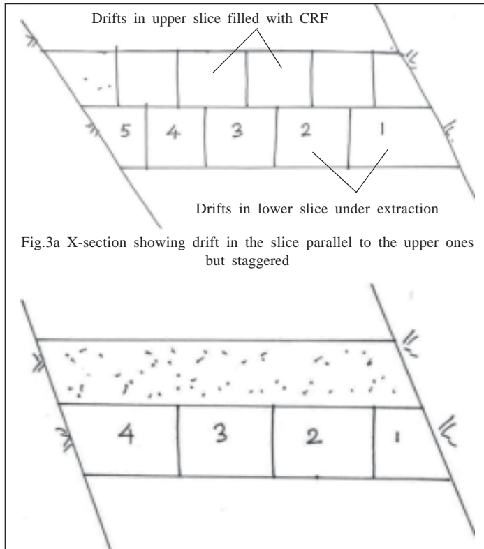
Fig.3b X-section showing drift in the slice at angles to the upper ones
