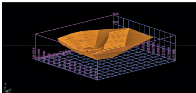
Figure 5: Pit design
