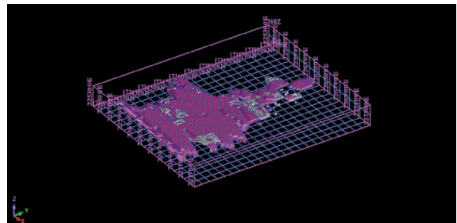
Figure 4: Solid ore block model constrained with attributes by colors
