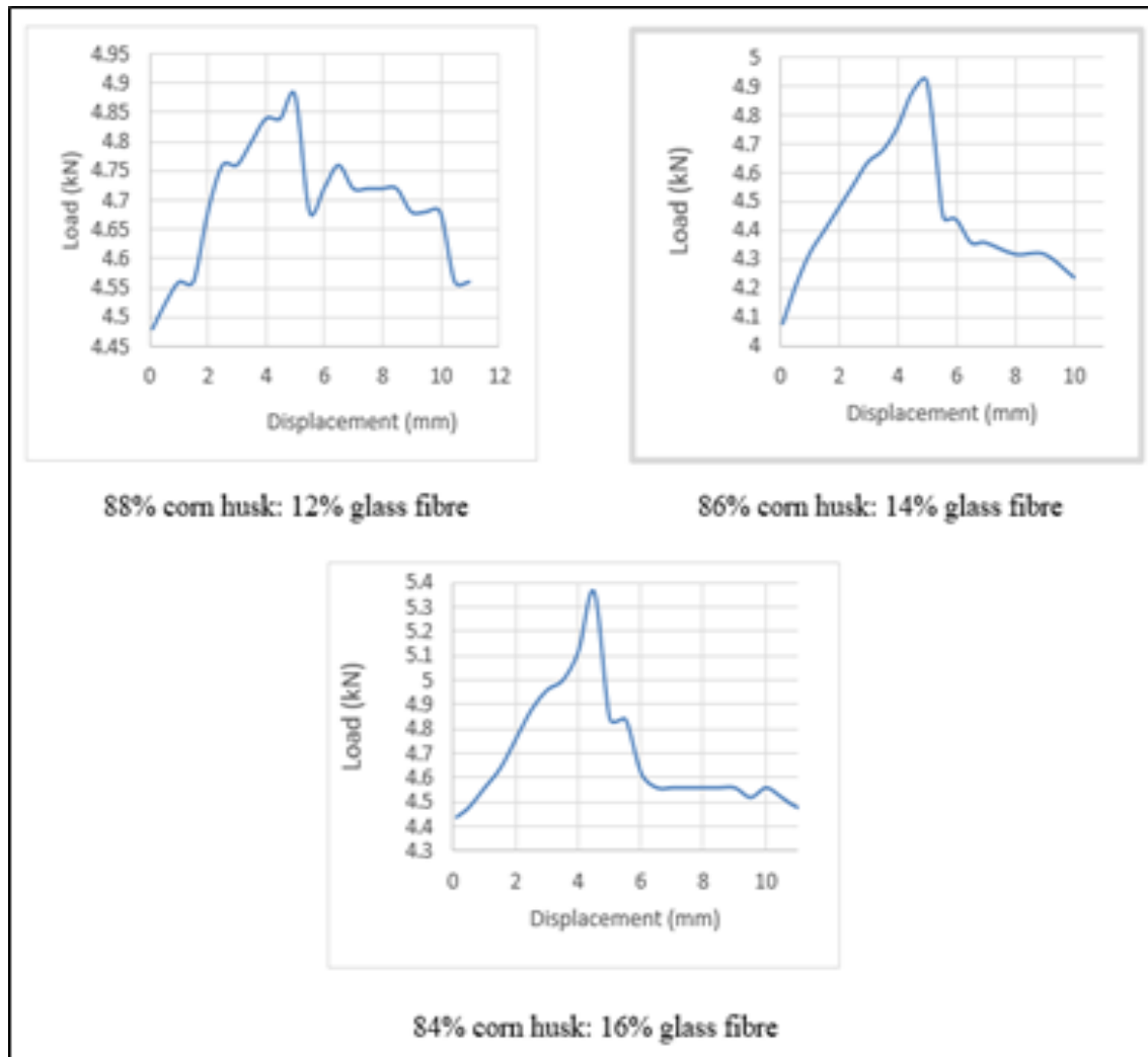
Figure 5. Load (kN) v/s Displacement (mm) - Bending test.
