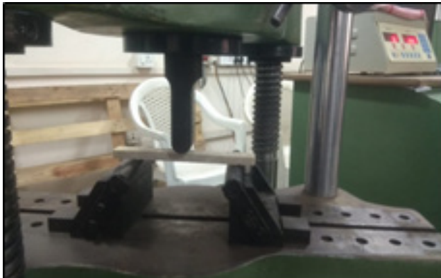
Figure 1. 3 Point bending test.
