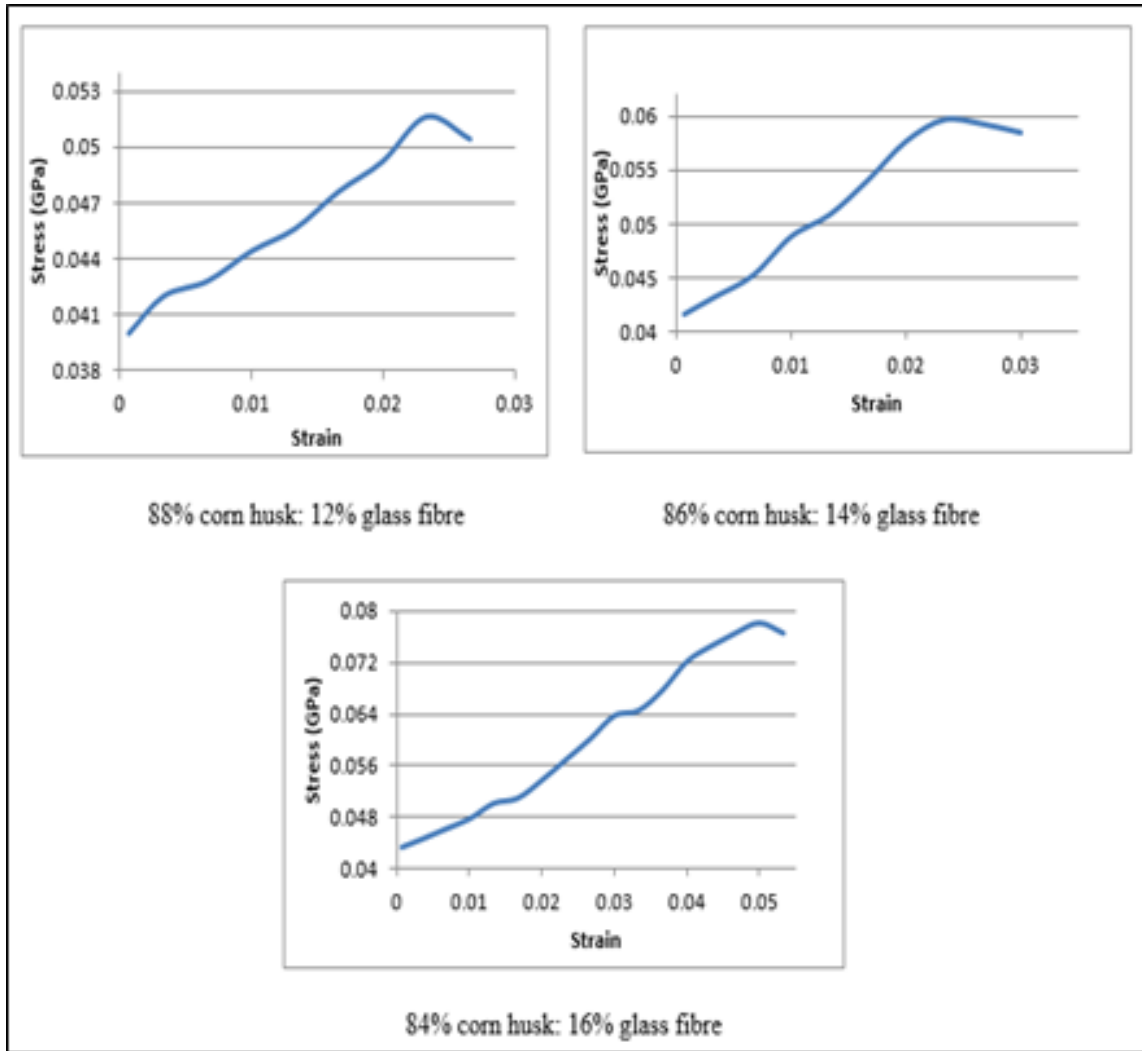
Figure 6. Stress (GPa) v/s Strain - Tensile test.
