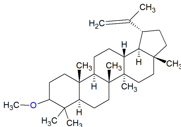
Figure 2. Probable structure of U1 (Lupeol Methyl Ether)(Calculated mol wt. 440.74398 g/mol).
