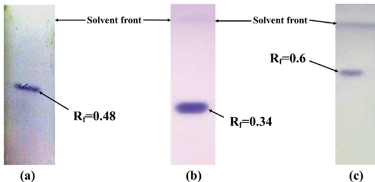
Figure 1. Purity assessment of isolated compound U1 in three different mobile phases. (a). Pet. ether: ethyl acetate: methanol: glacial acetic acid (6:4.5:0.5:0.2 v/v/v/v) (b). Pet. ether: ethyl acetate: methanol (6:3:0.4 v/v/v) (c). Toluene: ethyl acetate: methanol (7:3:0.5 v/v/v).
